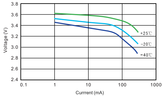
Voltage plateau versus Current and Temperature
